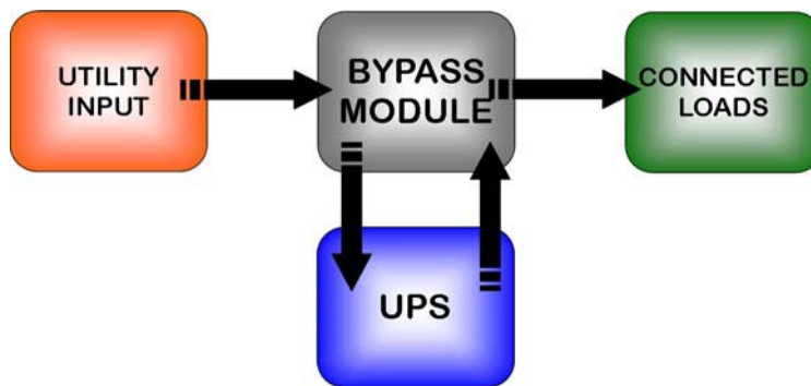
Figure 3: UPS MODE
